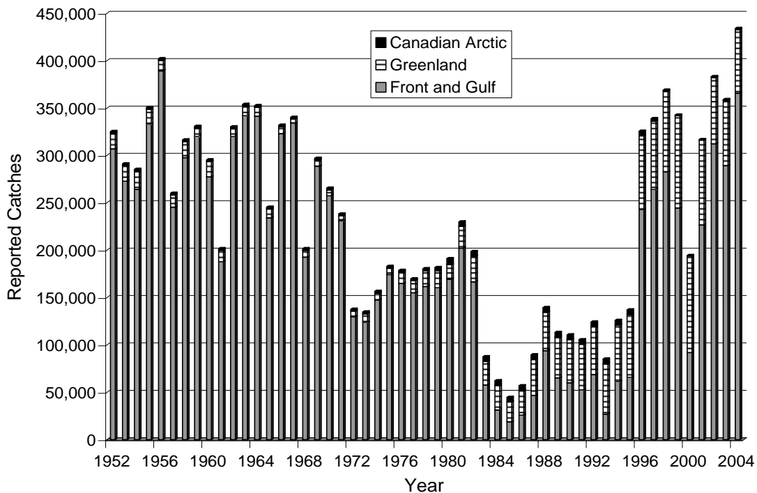
Figure 2: Reported commercial and subsistence catches of harp seals in the northwest Atlantic 1952-2004. Totals do not include seals killed but not landed or those killed as bycatch in commercial fisheries.
