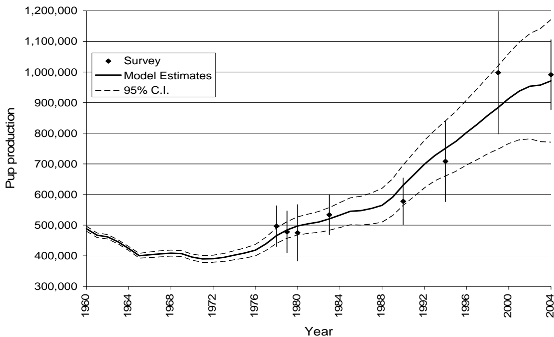
Figure 3: Independent survey estimates (bars indicate 95% confidence intervals) and model estimates of pup production 1960-2004.
