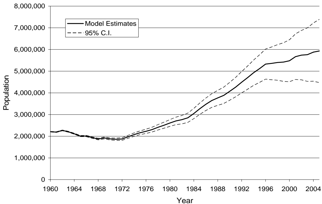
Figure 4: Estimates of total population 1960-2004.
